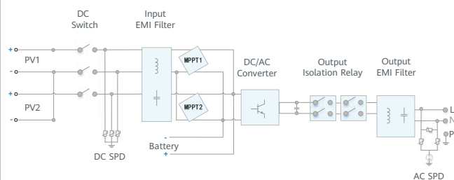
Circuit Diagram
